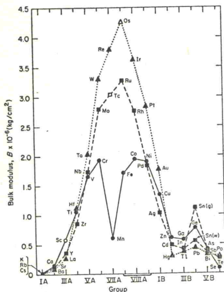
FIG. 6. Bulk modulus of the elements of the fourth, fifth, and sixth periods of the Periodic Table. Open points are estimated values.
